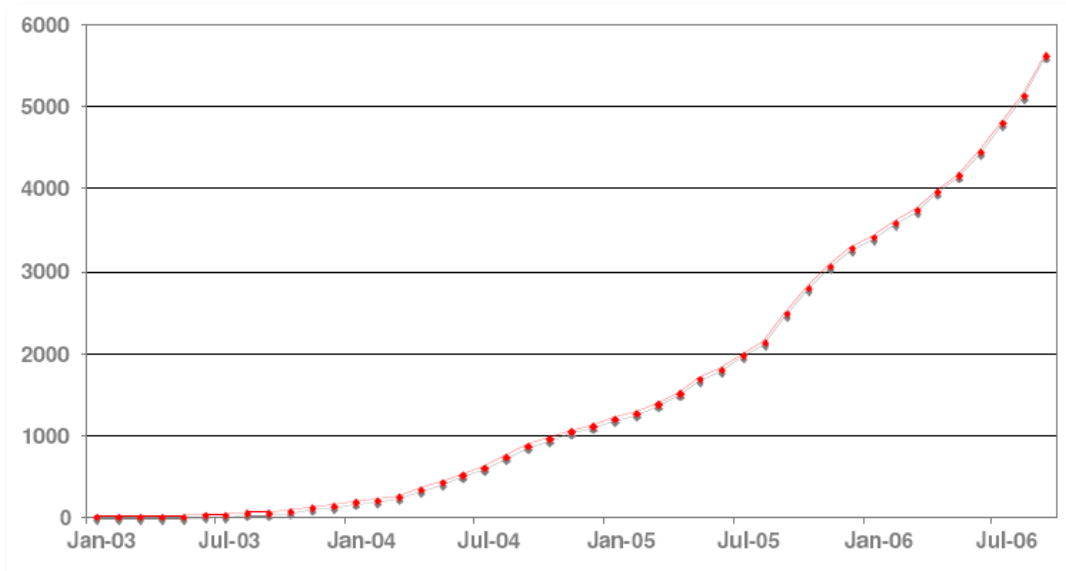
Growth of MapReduce Programs in Google Source Tree (2003 – 2006) (Implemented as C++ library)
